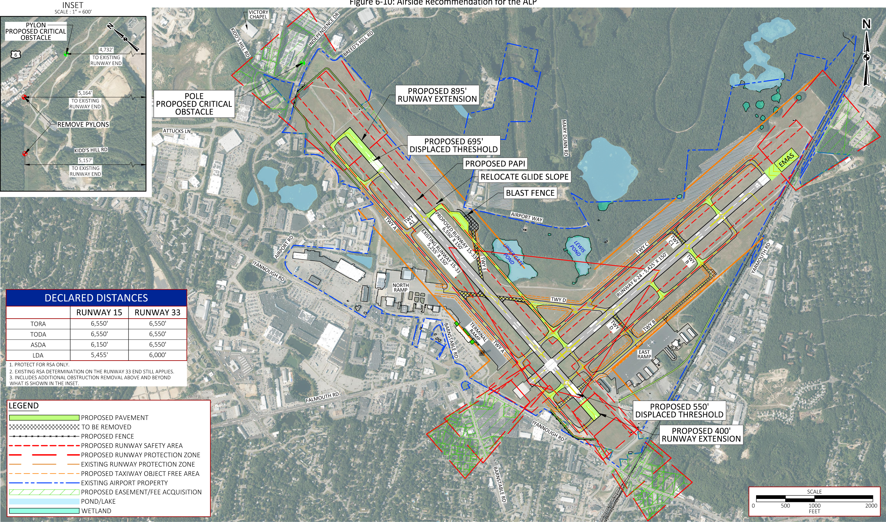
Figure 6-10: Airside Recommendation for the ALP
